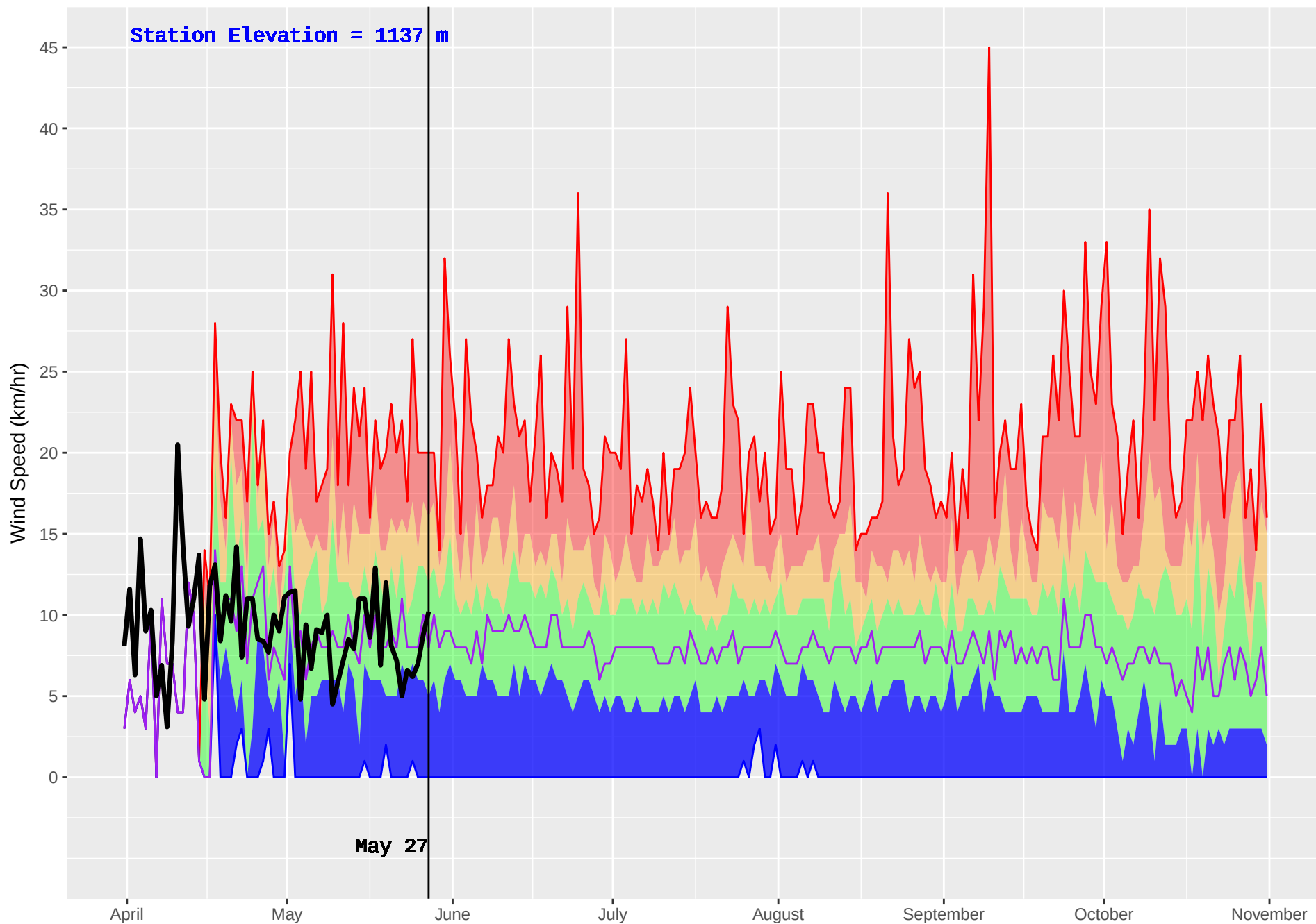
KLUSKUS (166) : Historical (1982–2016) and Current (2018) Noon Wind Speed
